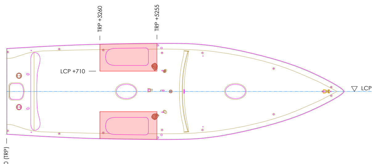
Figure 9.1: Cockpit modification areas
