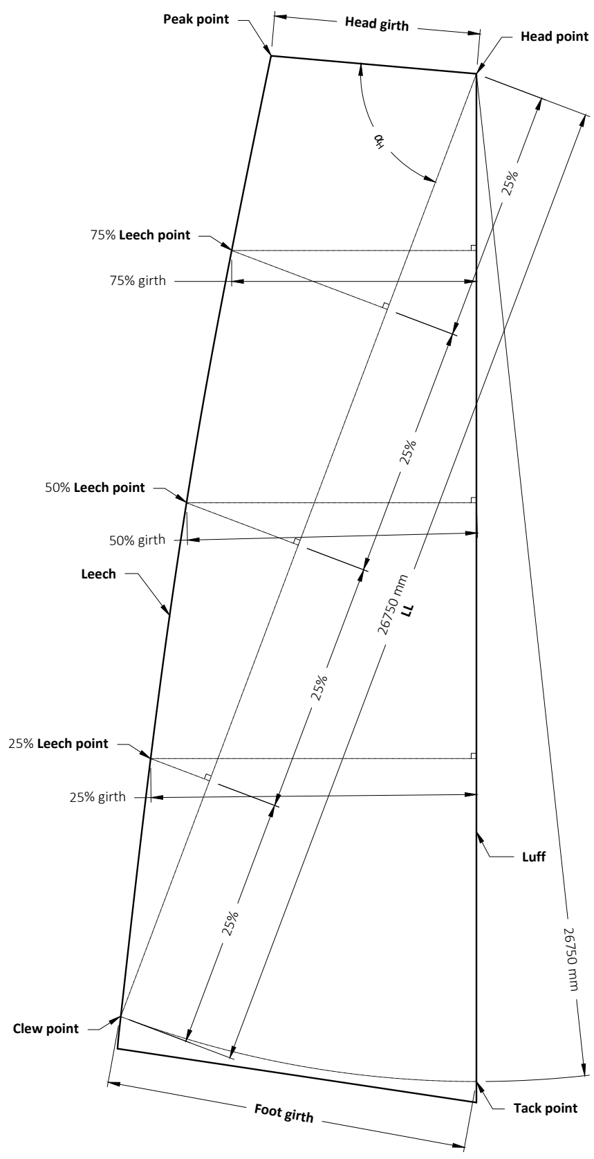
Figure 19.2: Mainsail Measurement
